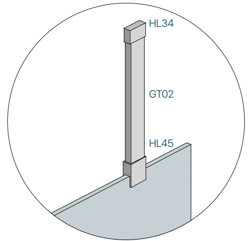
PCA-HL45 Glass - Track Holder 8,10mm | Glass Thickness Stainless Steel 304 | Material Satin, Polished | Finish
