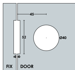
Glass Cut
