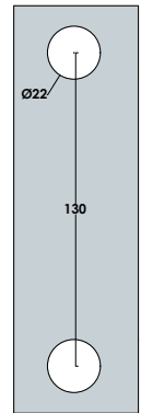
Glass Preparation
