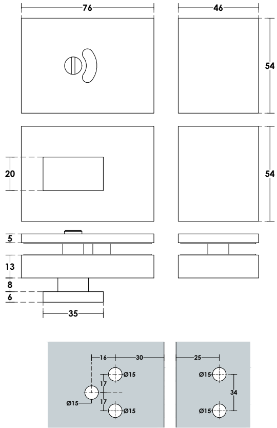
Glass Cut
