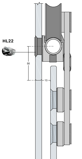
Skylight installation
