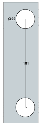
Glass Preparation
