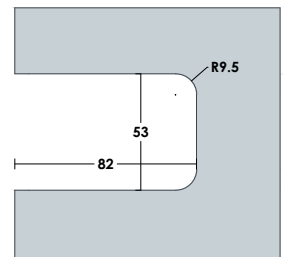
Glass Cut
