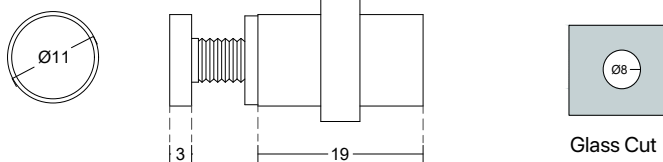
PCA-HR06 Self Holder 5-10mm | Glass Thickness Zinc Alloy | Material Satin, Polished | Finish
