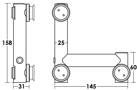
Glass Cut
