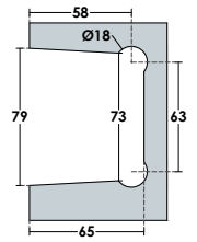
Glass Cut
