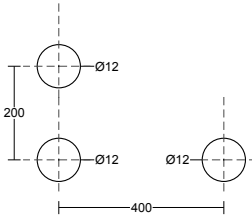
Glass Cut
