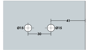
Glass Cut
