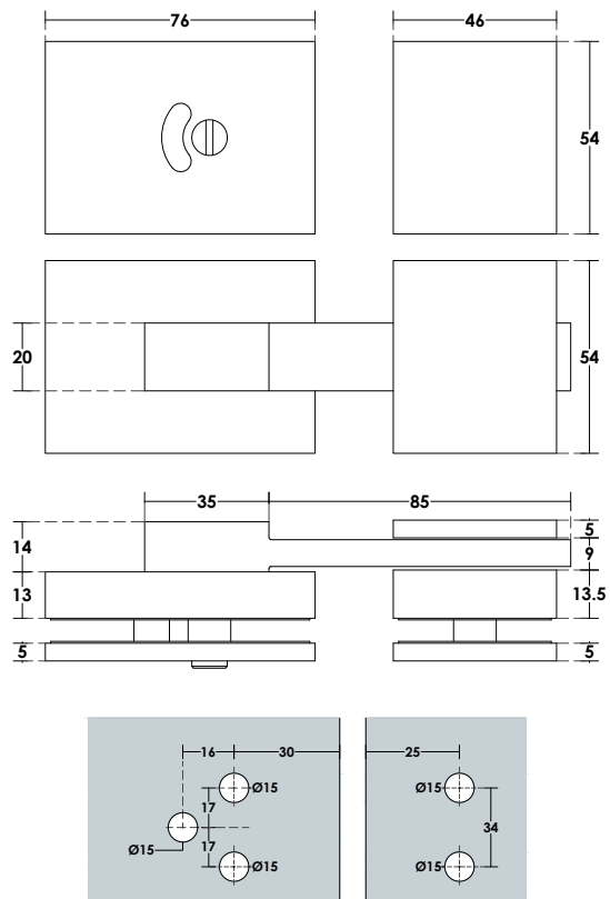
Glass Cut
