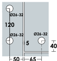
Glass Cut
