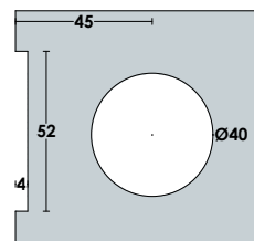
Glass Cut
