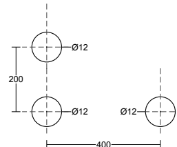
Glass Cut
