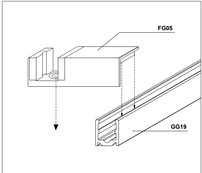
Waterproof bottom track option
