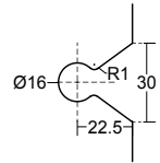
Glass Cut
