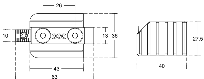
GG08-U Connection
