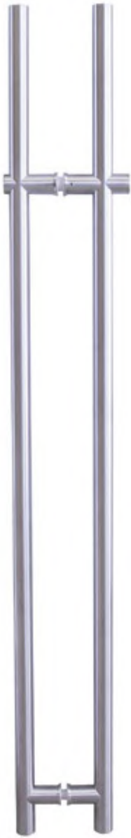
PCA-HD06 Door Lock - Handle Ø35mm 10-12 mm | Glass Thickness Stainless Steel 304 | Material Satin | Finish
