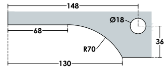
Glass Cut
