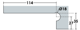
Glass Cut
