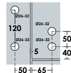
Glass Cut
