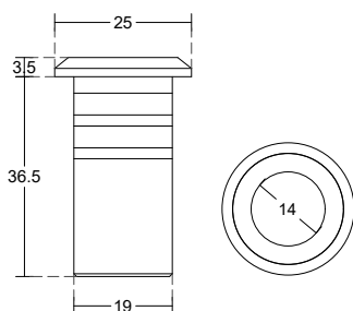
PCA-KP01 Floor Socket Stainless Steel 304 | Material Satin | Finish
