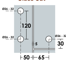
Glass Cut
