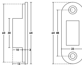
Magnetic Strike Plate
