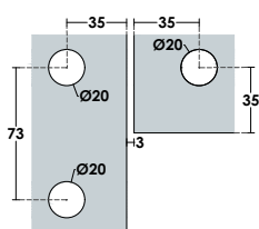
Glass Cut
