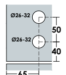
Glass Cut
