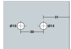
Glass Cut
