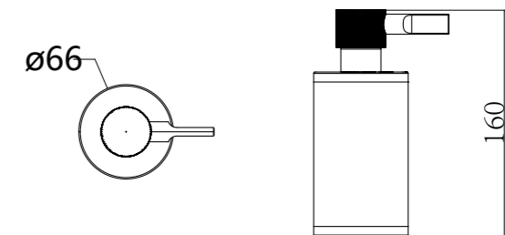
NUCCIA-04 SR-06.29.199.05 Soap Dispenser | Product Brass and Stainless Steel [304] | Material Colours Available:
